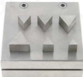
DSC-044 6pc Equilateral Triangle Disc Cutter Set Cut Sizes: 4, 8, 10, 12, 14, 18mm Material: Steel Available with Allen Key Tool or Locking Lever
