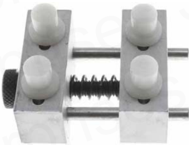
WMH-001 Small Adjustable Watch Movement Holder, 12 Holes Aluminum Body 4pc Pins With Nylon Head 12 Holes Holds Up To 1" Movement
